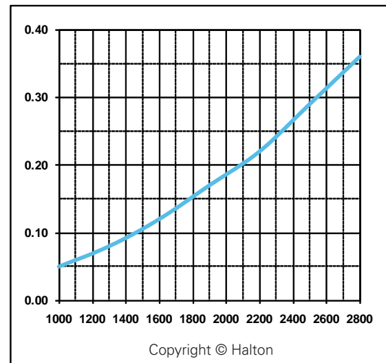
KVW/KVO/KVR - 3.5 Filters Per Side
