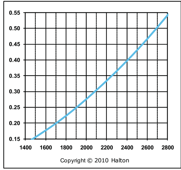
KVE/KVC- 5.5 Filters
