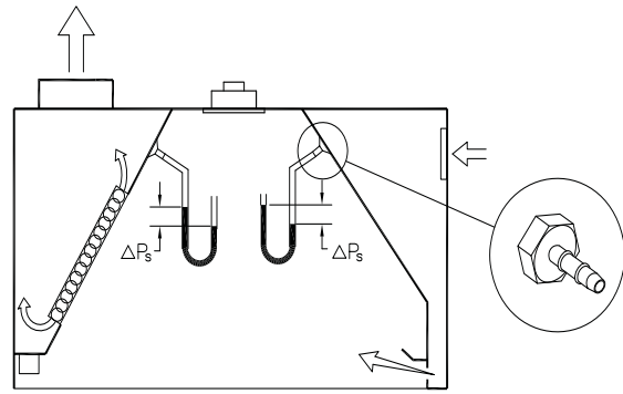
Exhaust air flow vs. pressure differential
