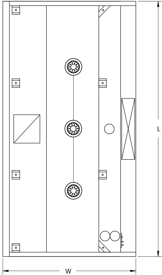
Mounting bracket 2" high (52mm)
