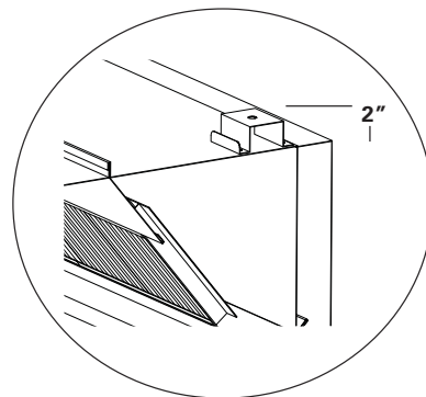
Mounting bracket 2" high (52mm)
