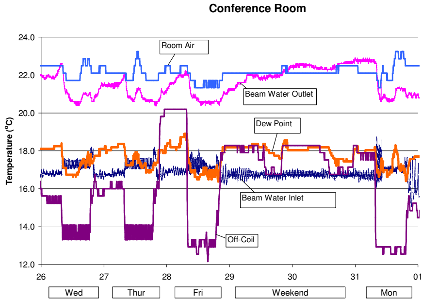
Figure 2. The operation temperatures in the conference room during six days.
