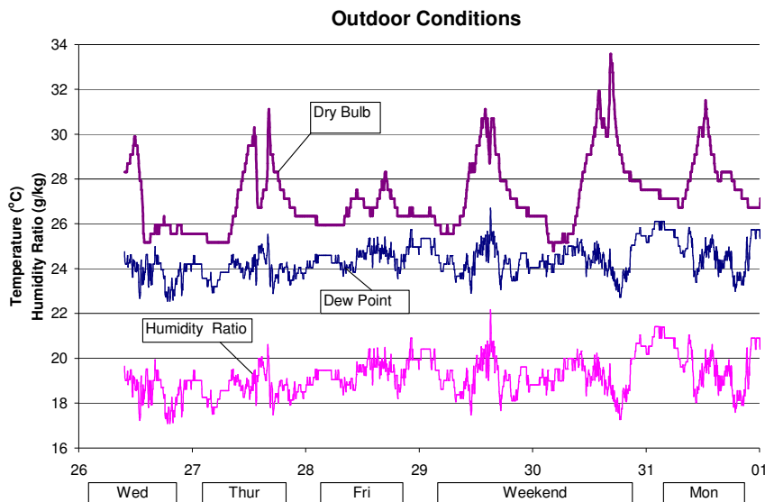
Figure 4. The outdoor conditions during measurement period of six days.
