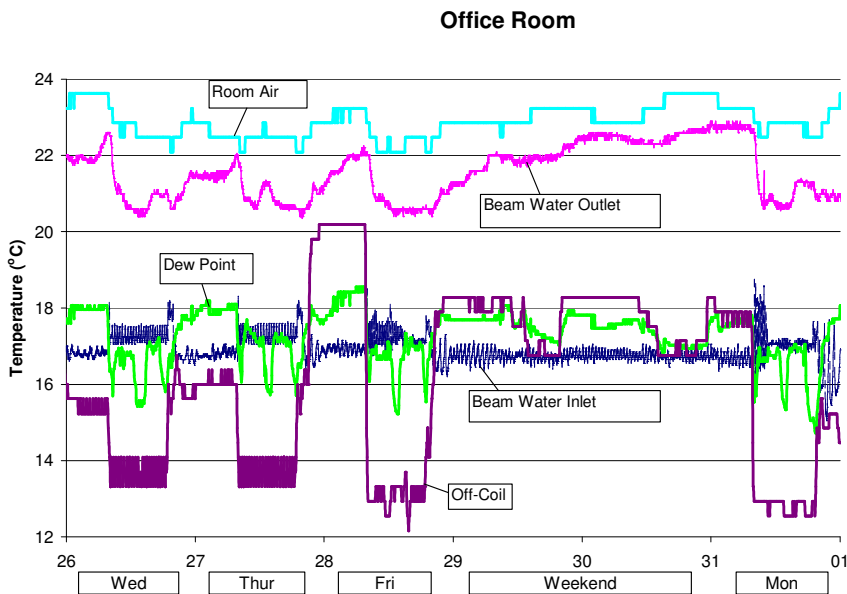
Figure 3. The operation temperatures in the office room during six days.
